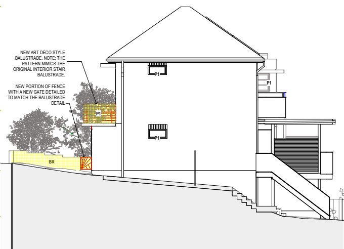
4 PROPOSED SOUTH ELEVATION 1:200
